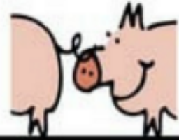
LITTLE-ENDIAN
